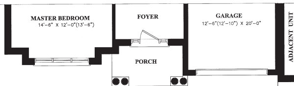
PART FIRST FLOOR PLAN ELEVATION "B"
