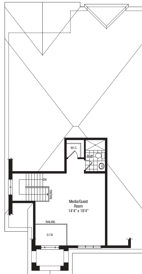
Loft Plan Elevation A
