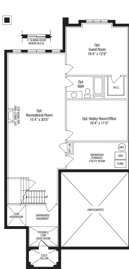
Basement Floor Plan Elevation A
