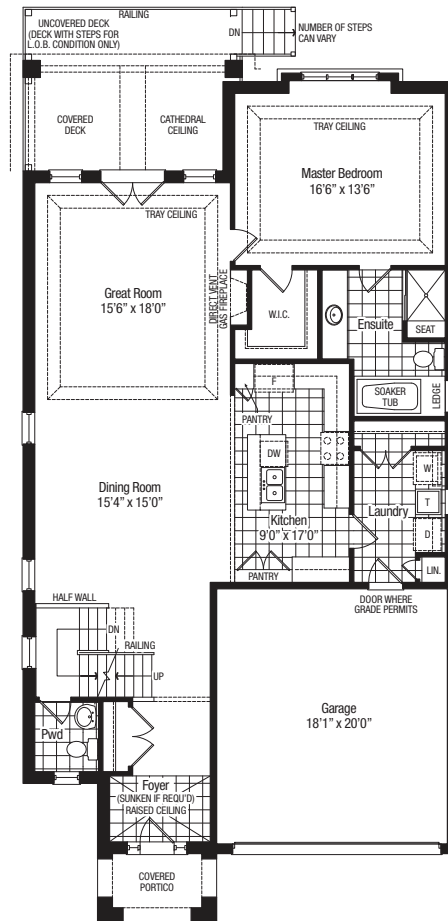
First Floor Plan Elevation A
